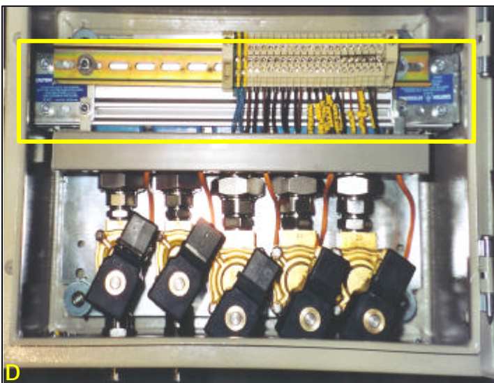
D,E: Biogas (Spain) - Modulair manifolds feeding a group of pneumatic valves.
